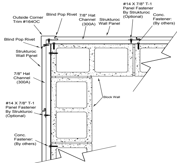
Detail @ Outside Corner with Hat Channel Note: Hat Channel is to be used @ 5' 0" O.C. Max.
