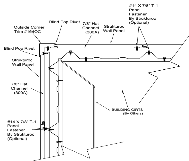
Detail @ Outside Corner with Hat Channel Note: Hat Channel is to be used @ 5' 0" O.C. Max.
