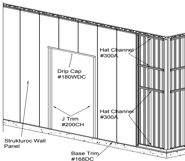
Detail @ Door Opening with Hat Channel Note: Hat Channel is to be used @ 5' 0" O.C. Max.
